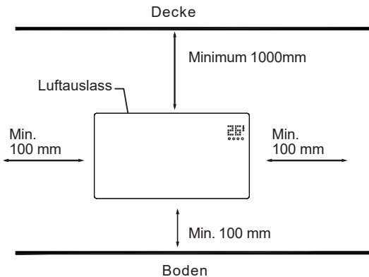
Wandmontage
