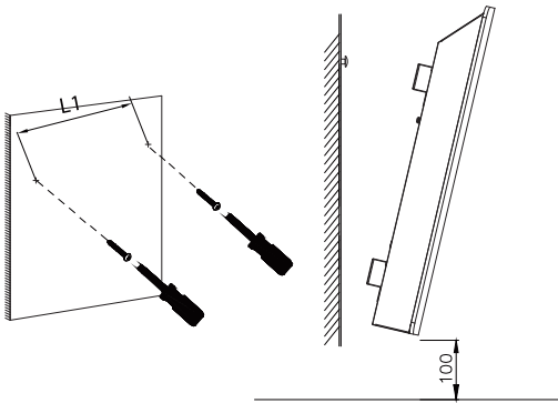
Wandmontage
